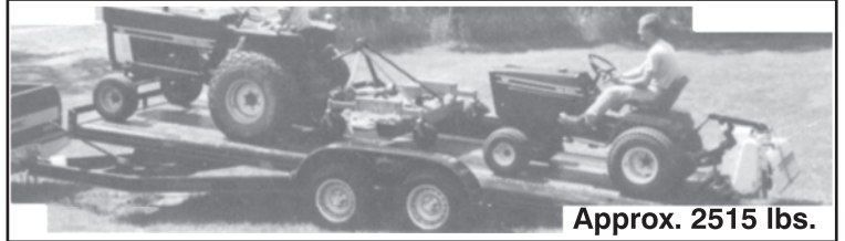
Picture shows 20' Excursion 10000 G.V.W. hyd. tilt lowboy
